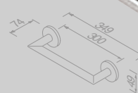
Badgreep 30 cm Grab rail 30 cm 916506-05
