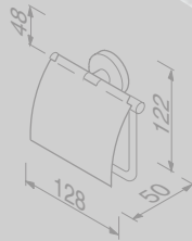
Toiletrolhouder met klep Toilet roll holder with cover 916508-02
