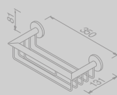
Douchemand 30 cm Shower basket 30 cm
