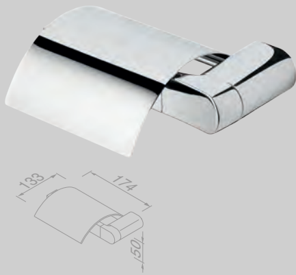
Toiletrolhouder met klep (links) Toilet roll holder with cover (left-handed) 914508-02-L
